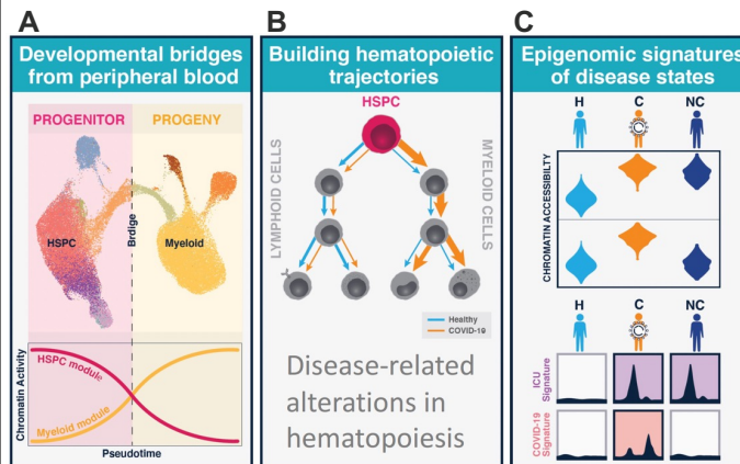
Figure 1: Proof of concept application of PBMC-PIE to a cohort of COVID-19 patients and controls recovers the developmental trajectory of myeloid cells originating from (A) HSPCs, (B) identifies disease-related alterations in hematopoiesis, and (C) reveals epigenetic signatures of HSPCs associated with disease states.
